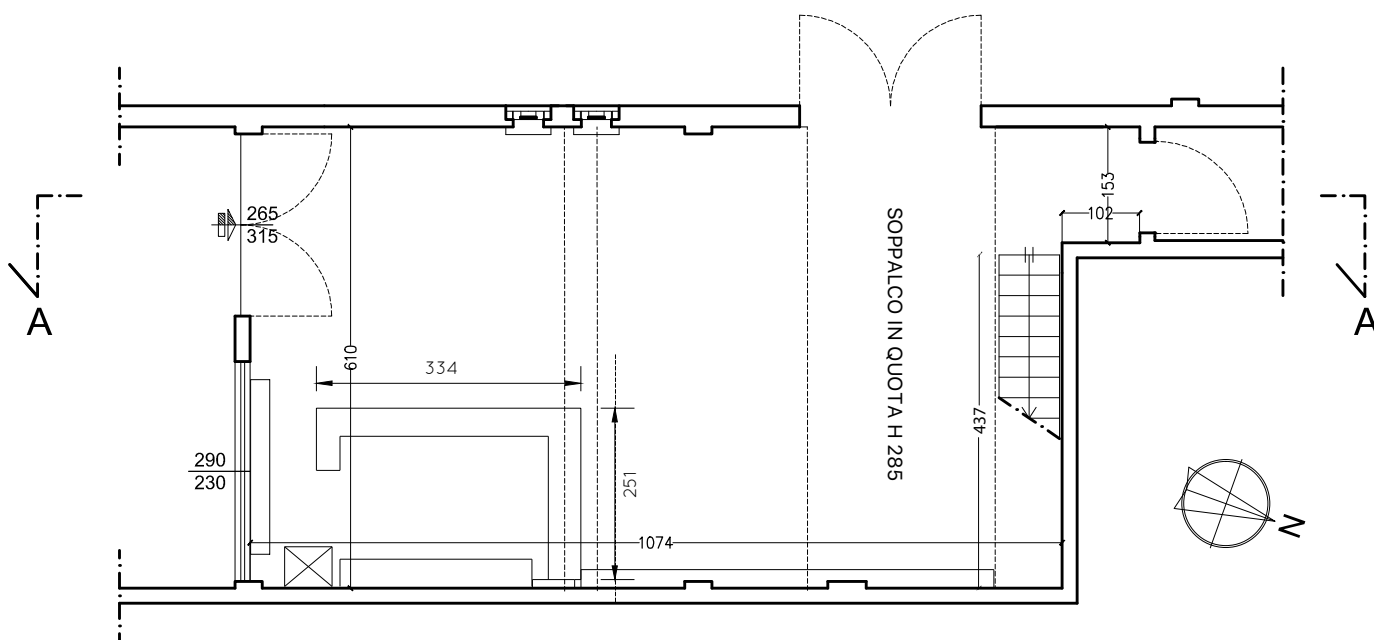
PIANO TERRA
